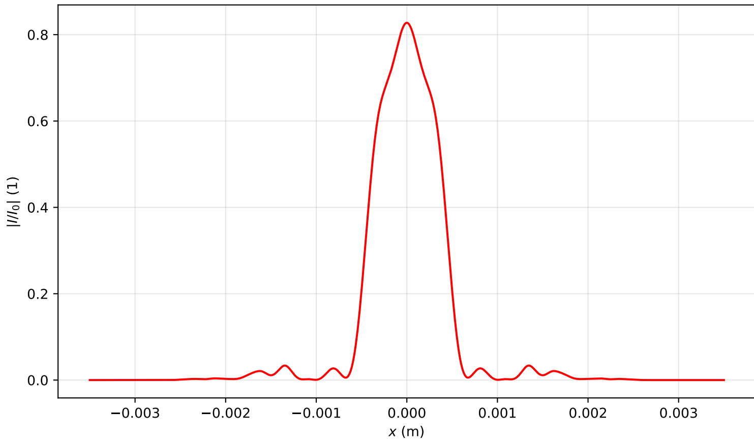
Intensity profile I(x, y = 0, z = 2.149)/I_0 , P_{in}=3.0P_{cr} , artificial time
